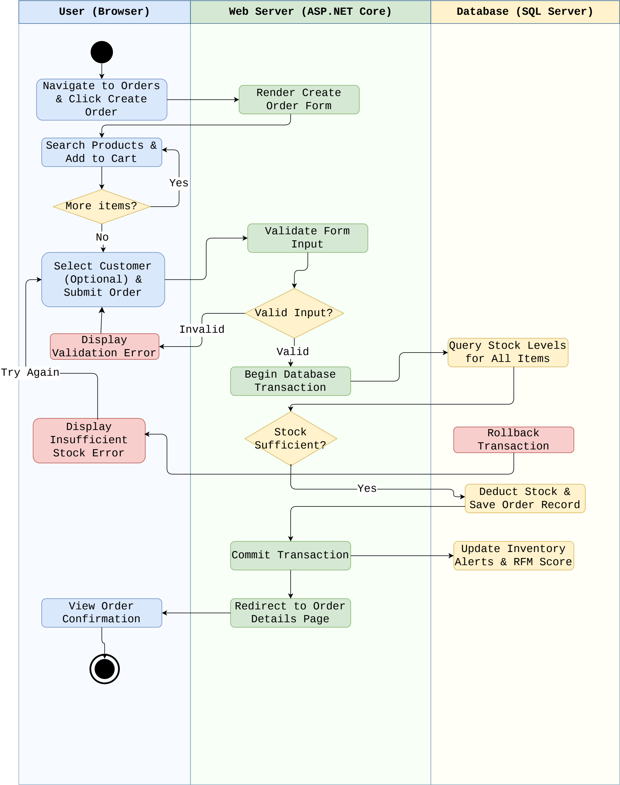
SellWise - Activity Diagram: Order Creation
